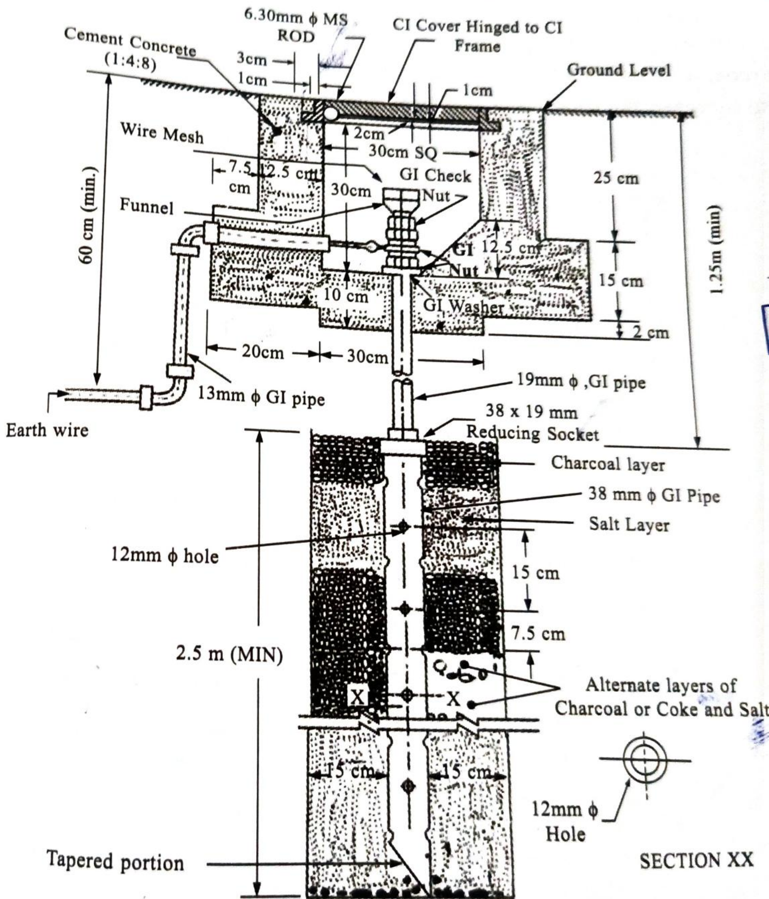
Fig 3.23 : Pipe Earthing
