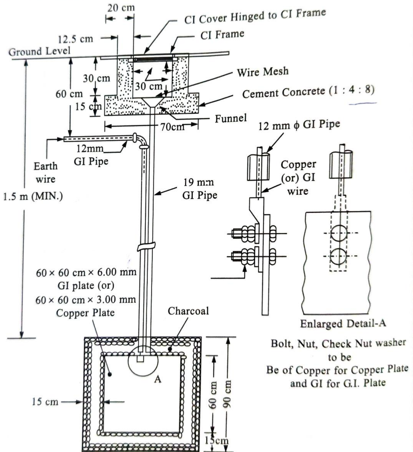
Fig 3.24 : Plate Earthing
