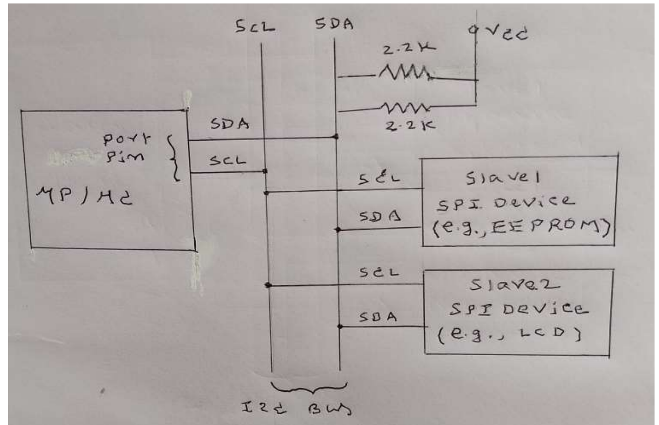
I2C Bus Interfacing
