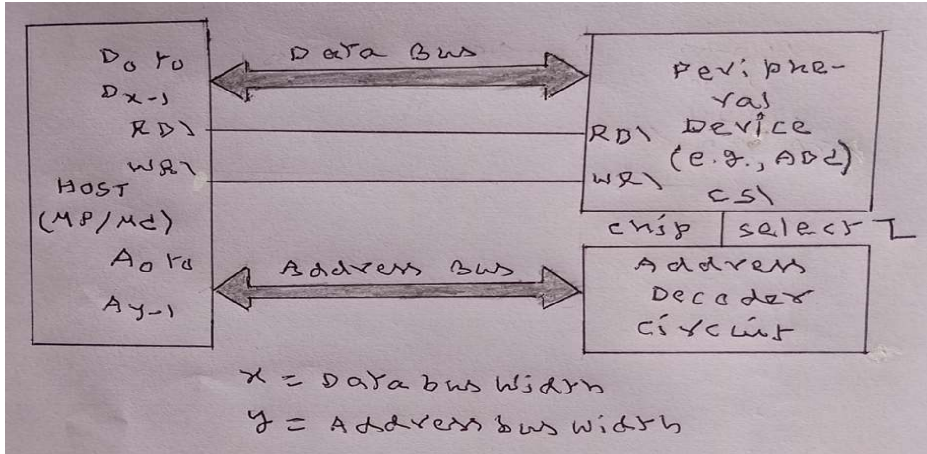
Parallel Interface bus
