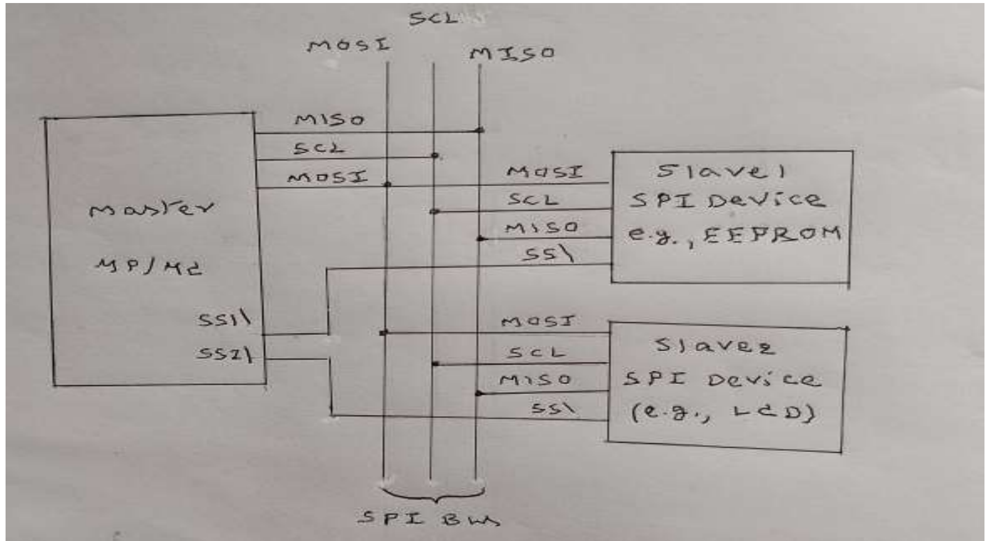
SPI Bus Interfacing
