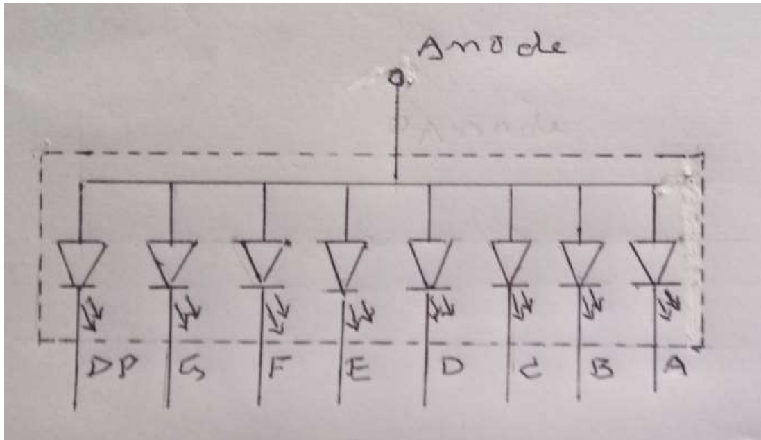
Common Anode Display
