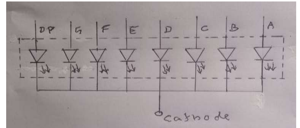
Common Cathode Display
