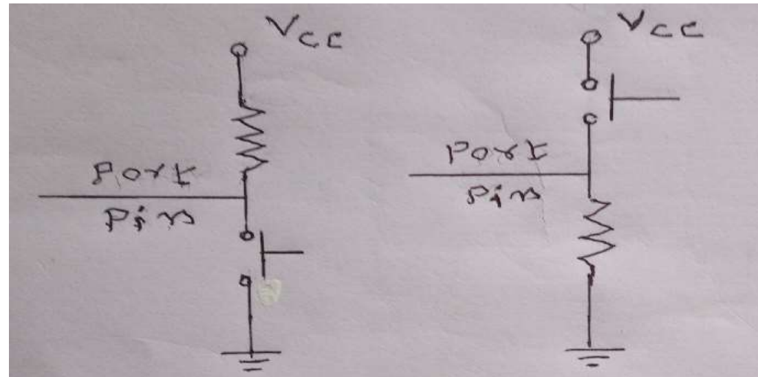
Fig. 5 (a): ‘LOW’ Pulse Generator
