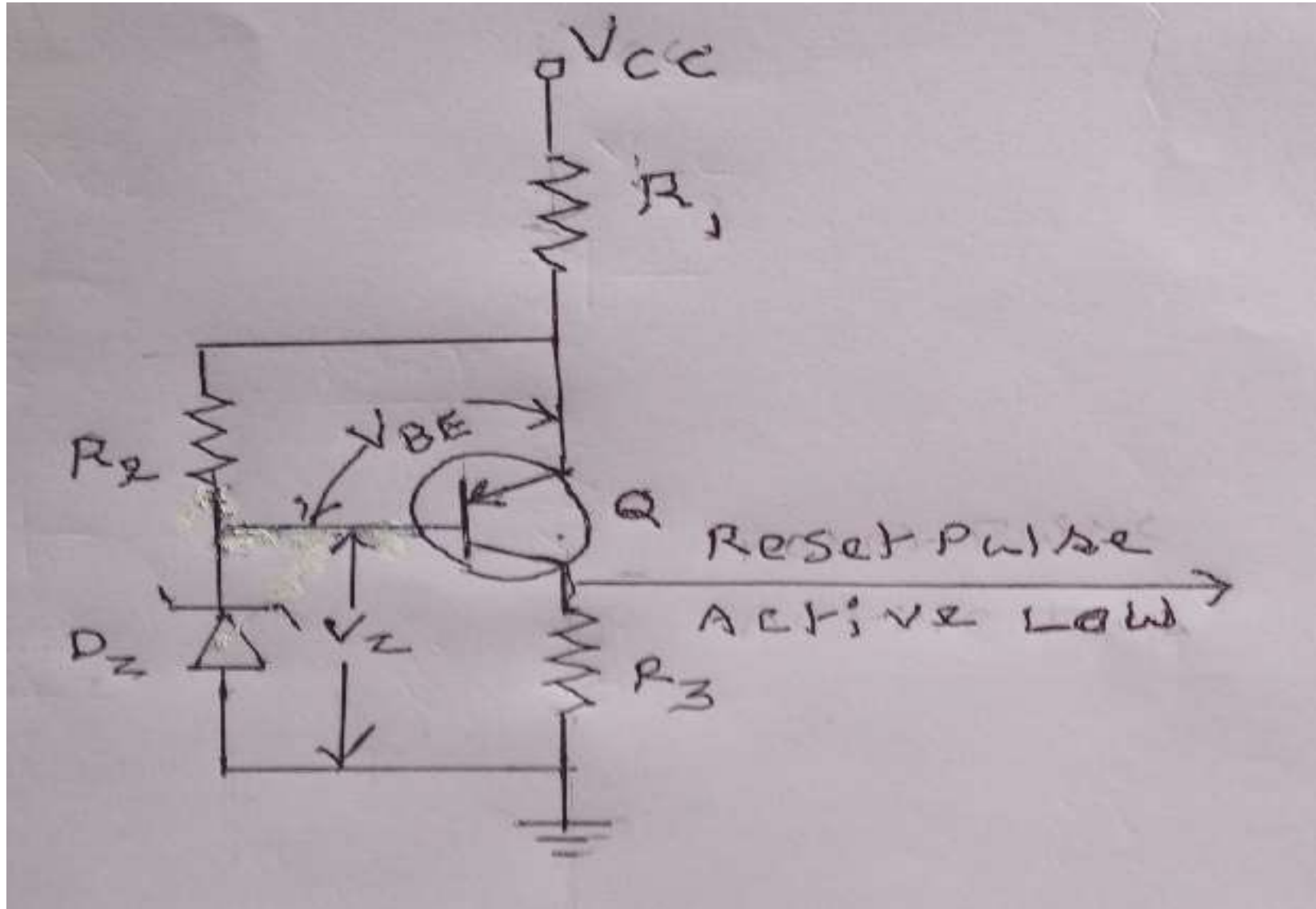
Brown-out protection circuit with active low output
