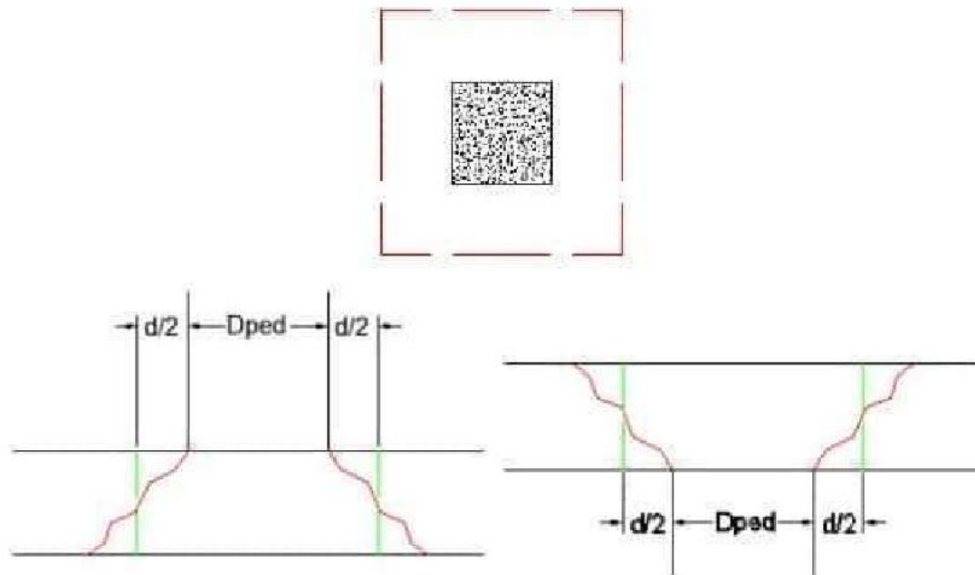
Fig.1. Punching Shear Failure Zone for Slabs above and below the column
