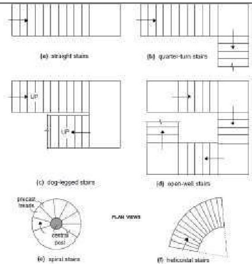
Fig. 2.11 Common geometrical configurations of stairs
