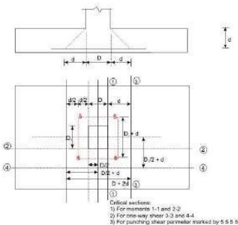
Figure 3.8: Uniform and rectangular footing
