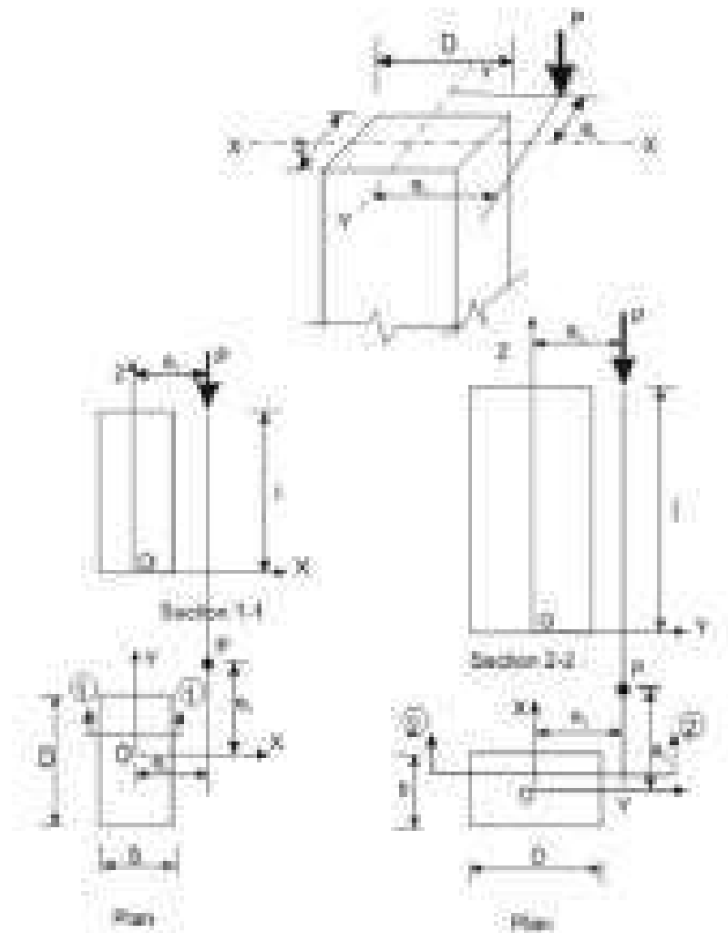
Figure 3.2(c) Axial loading with biaxial bending
